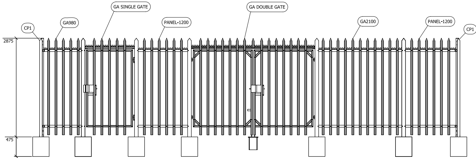
VIEW "A"
