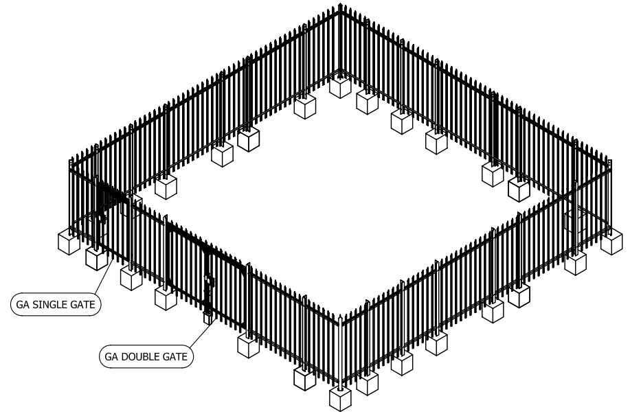
3D VIEW
