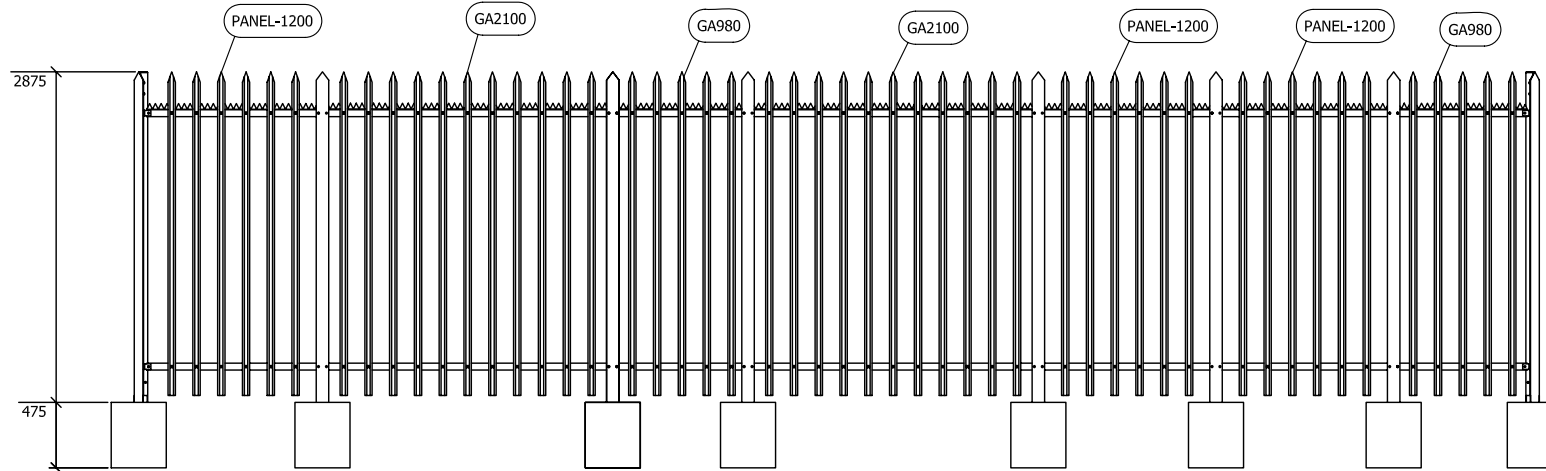
VIEW "C"
