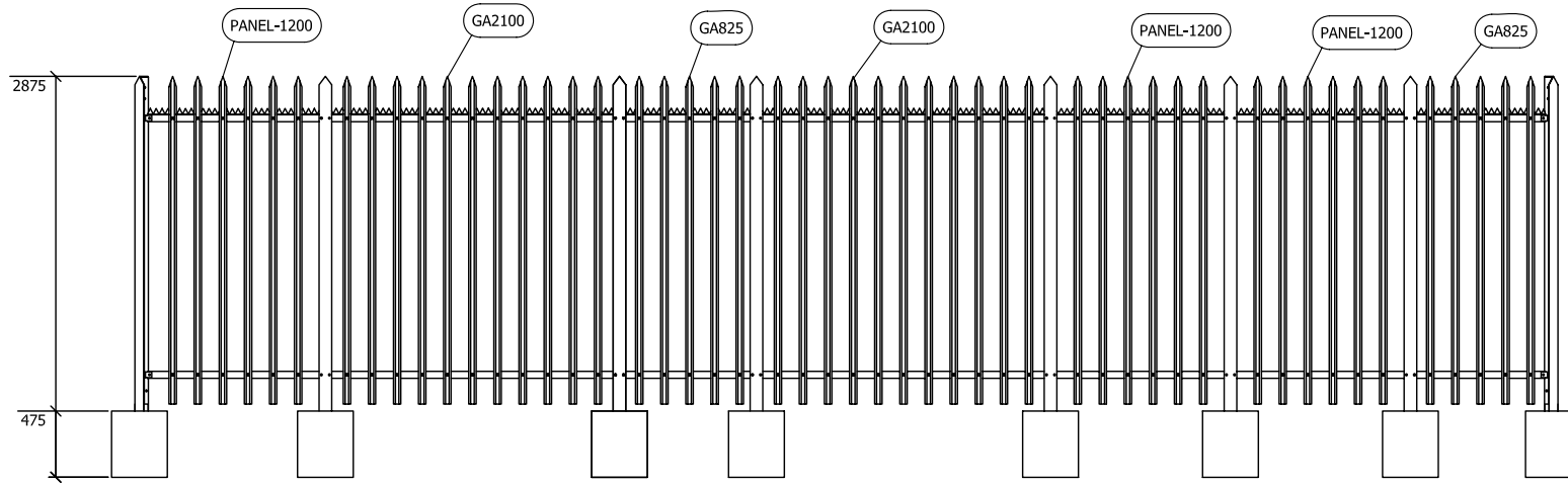
VIEW "B"
