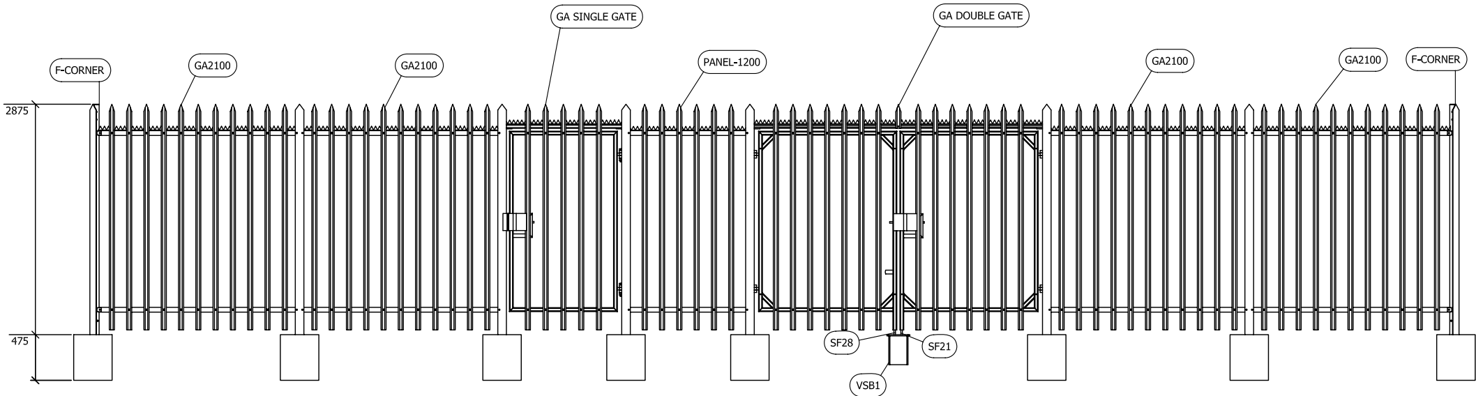
VIEW "A"
