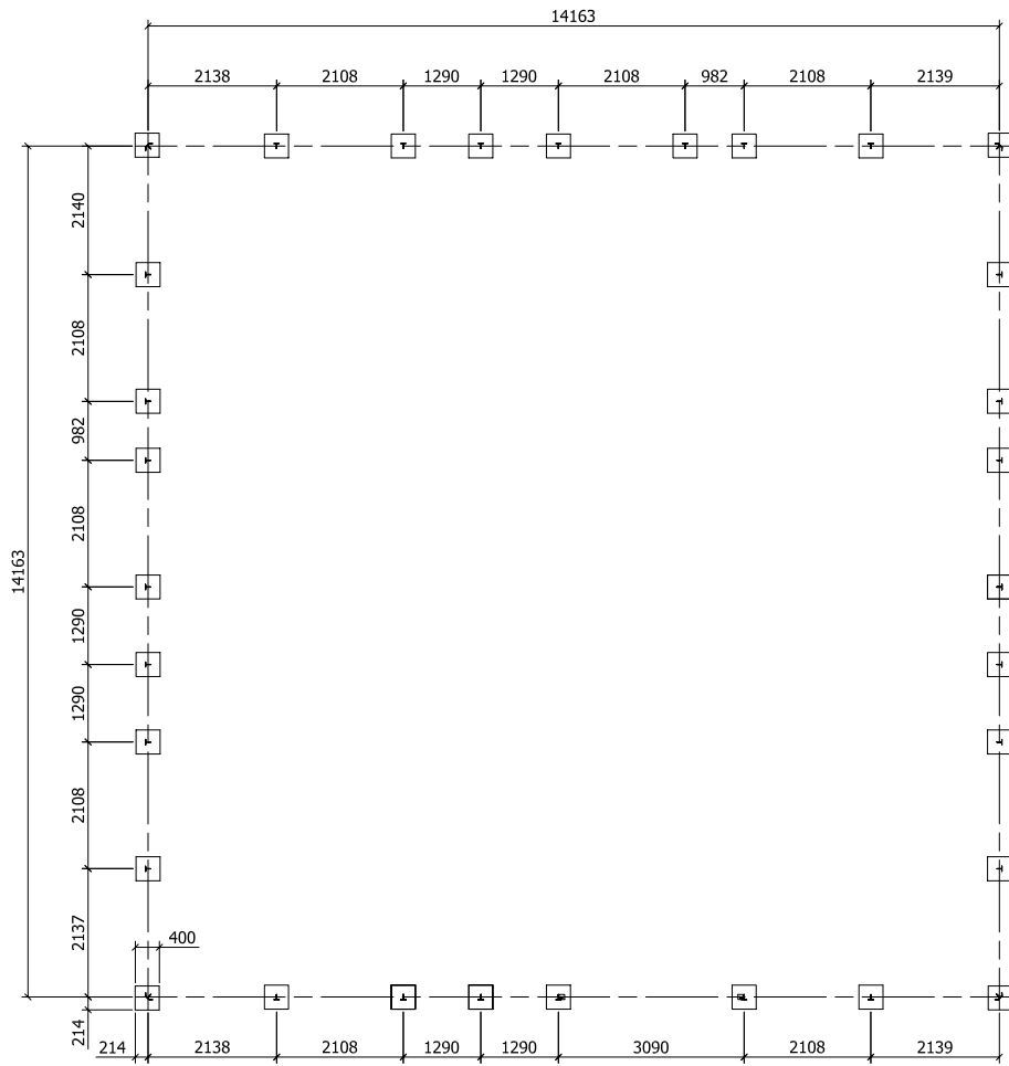
PLAN VIEW
